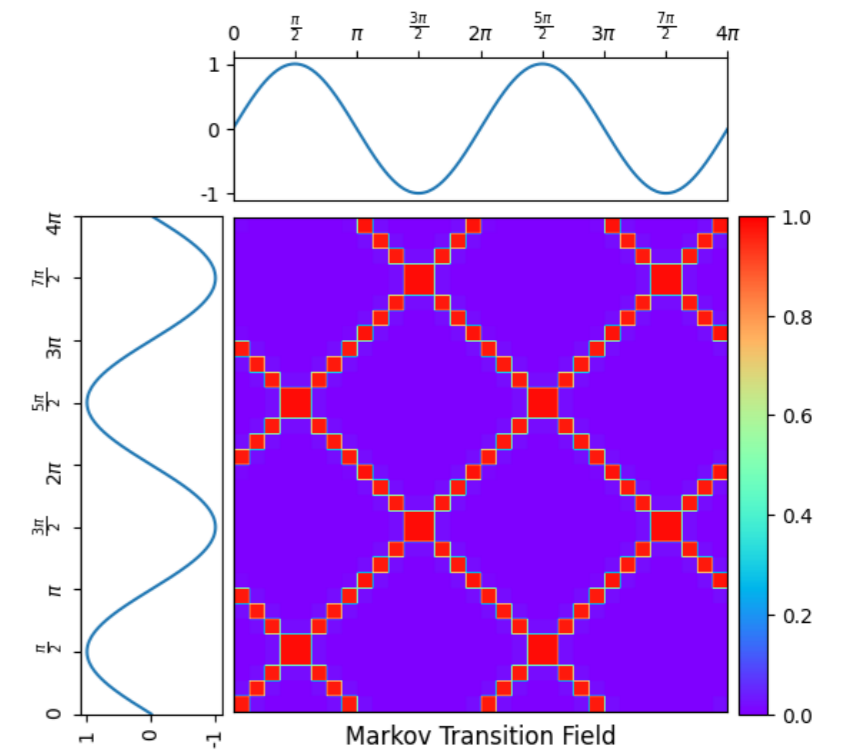
Markov Transition Field
