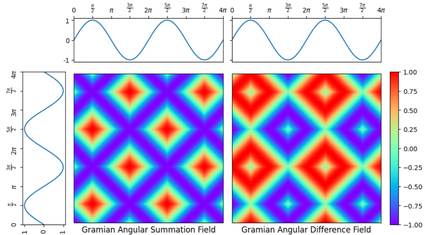
Gramian Angular Field
