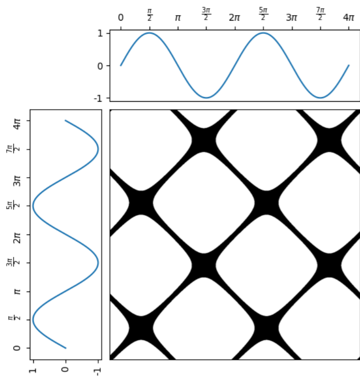
Recurrence Plot
