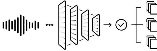
Classification
