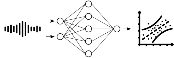
Regression
